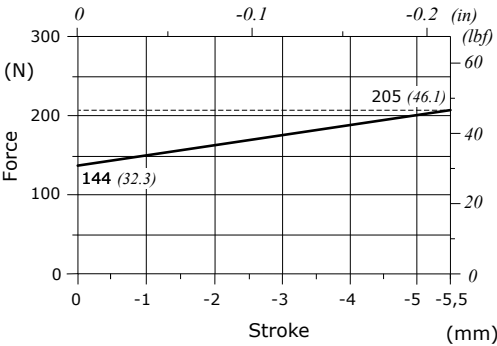
Force-Stroke diagram
