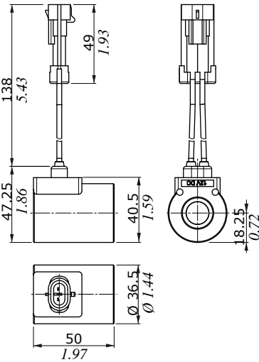
Flying leads with PACKARD METRI-PACK connector Flying leads with PACKARD WEATHER-PACK connector
