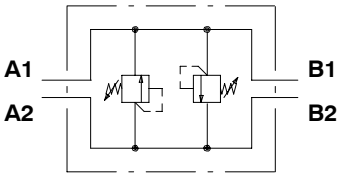
Configuration with valve on each workport (P3)
