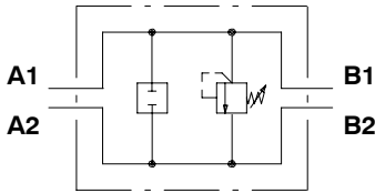
Configuration with valve on workport B (P1)
