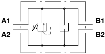
Configuration with valve on workport A (P2)
