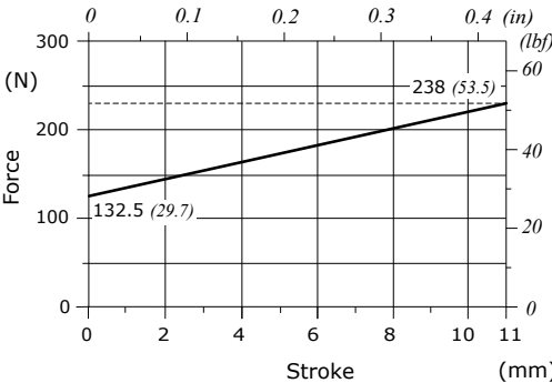
Force-Stroke diagram
