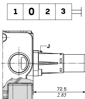
Type SLC With endcap
