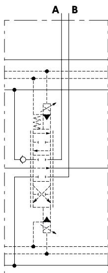
Type QE/Q5E Without port valves arrangement (type Q5E for floating circuit)
