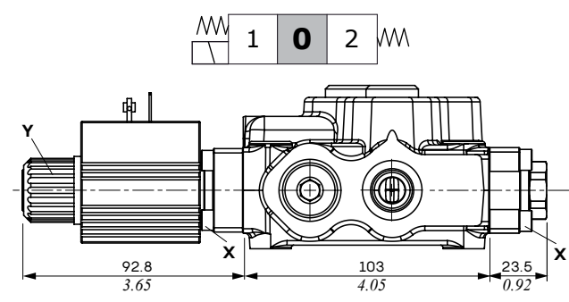
Type 8ES1 Single acting in A
