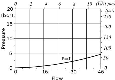
P⇒T pressure drops
