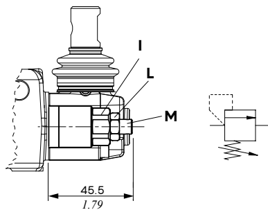
Type G configuration with screw
