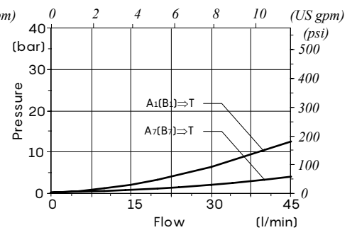
A(B) \Rightarrow T pressure drops 7 sections valve
