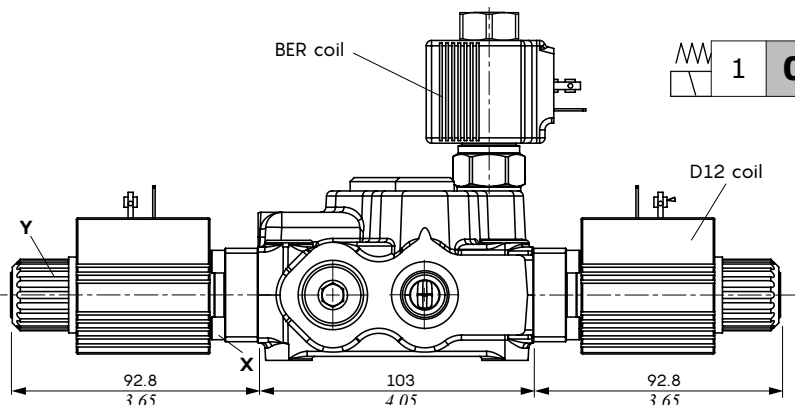
Type 8ES1 Single acting in A
