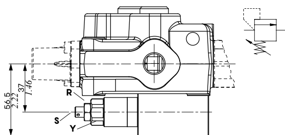
VSC valve
