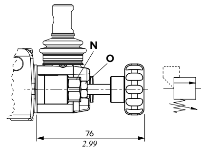
Type V configuration with handwheel
