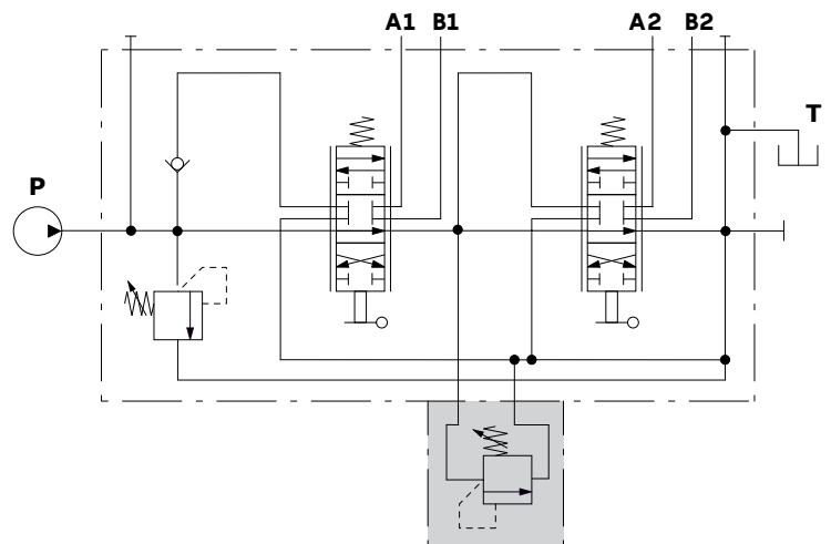
Hydraulic circuit with VSB
