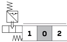
Type 8MS3 Switch in positions 1 and 2
