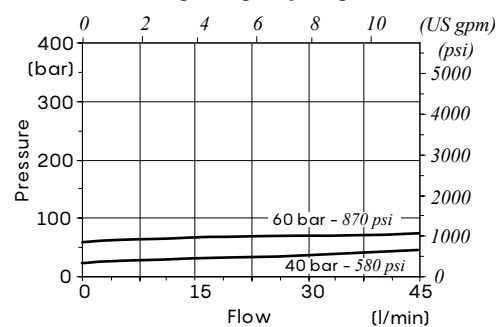
Setting range spring nr.2
