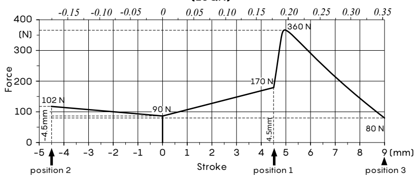
Force-Stroke diagram (13QN)
