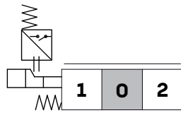
Type 8MS1 Switch in position 1
