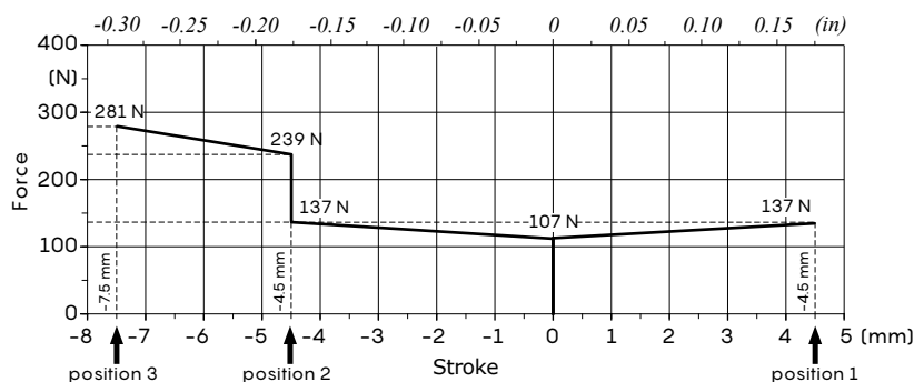
Force-Stroke diagram (13FZ)
