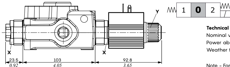
Type 8ES3LHE Double acting with manual override for emergency only
