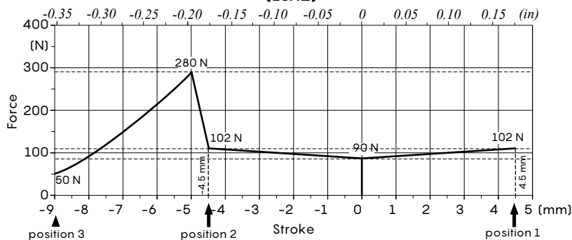
Force-Stroke diagram (13NZ)
