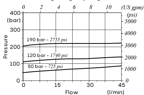
Setting range spring nr.3
