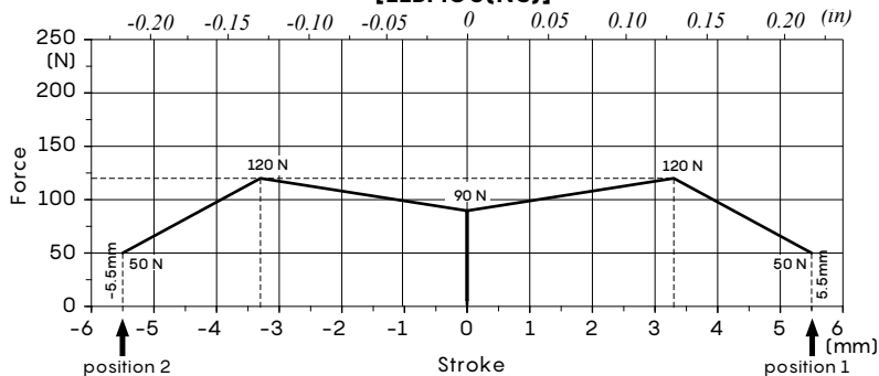
Force-Stroke diagram [11BMG3(NC)]
