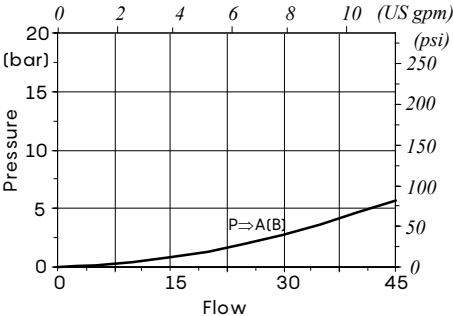
P⇒A(B) pressure drops 6 sections valve
