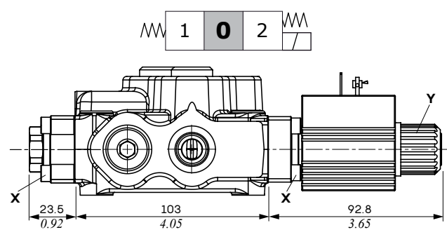
Type 8ES2 Single acting in B
