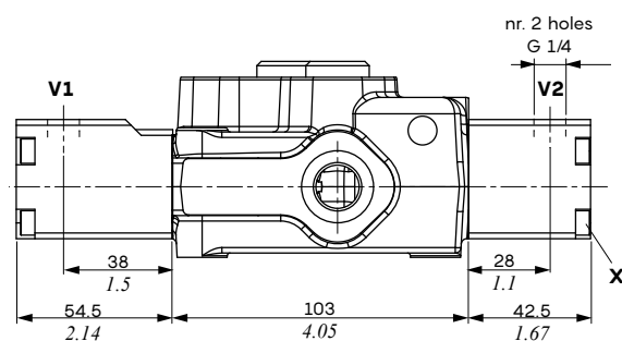
Type 13IM Pilot control kit for floating circuit for spools type 5DY
