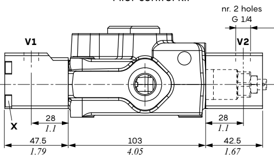
Type 8IM Pilot control kit
