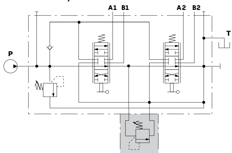
Hydraulic circuit with VSC valve
