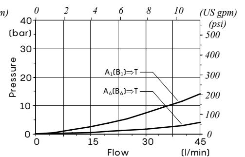
A(B) \Rightarrow T pressure drops 6 sections valve
