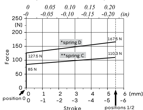
Force-Stroke diagram (8MG1-8MG2-8MG3)
